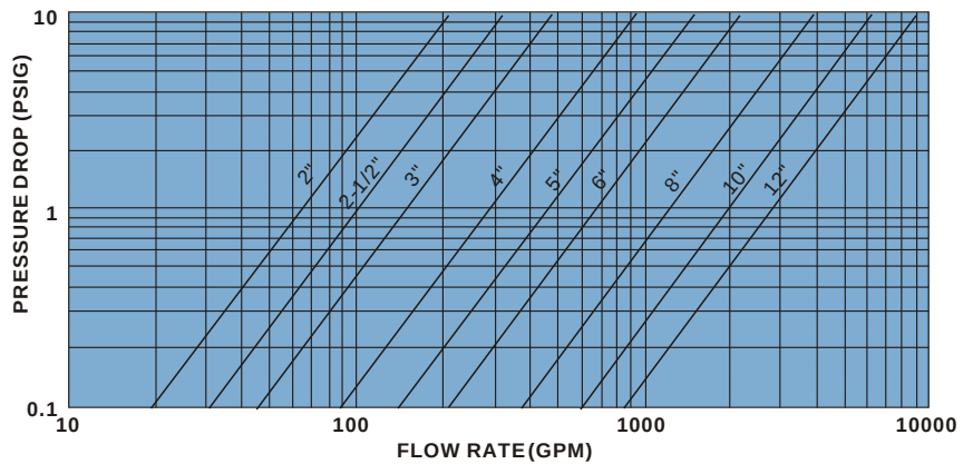
PRESSURE DROP VS FLOW RATE CLASS 300
