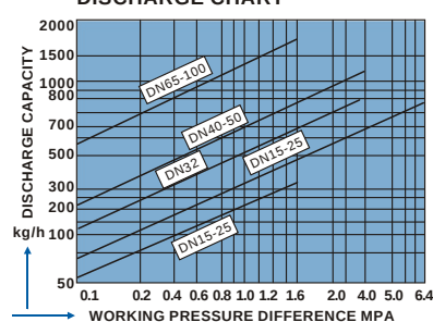
DISCHARGE CHART
