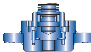
Pilot plug design from DN 200
