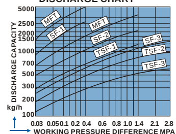
DISCHARGE CHART
